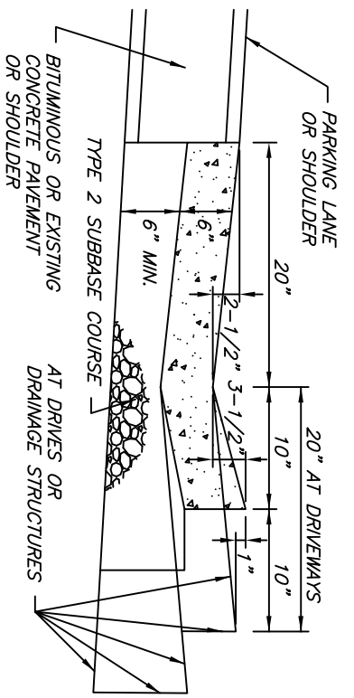
GUTTER SECTION #1 (PREFERRED)
